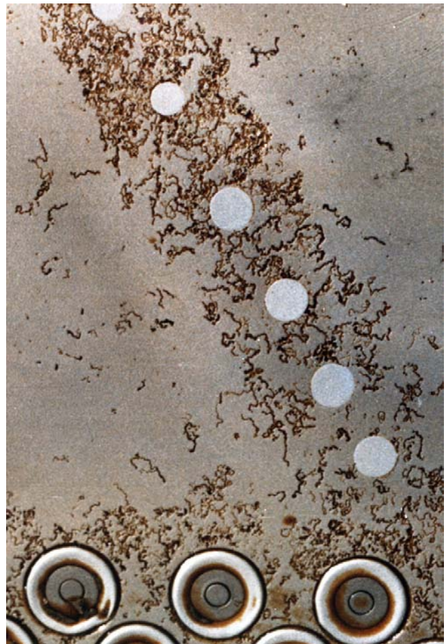
Figure 3-17. Filiform Corrosion Found Under Paint Coating on a Magnesium Panel
