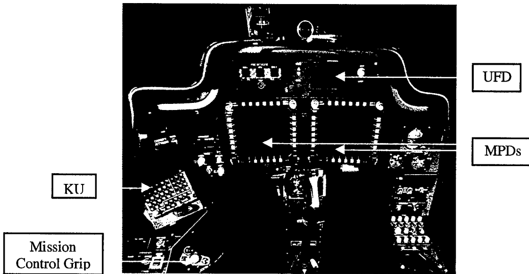
Figure 2. Pilot Crew Station.
